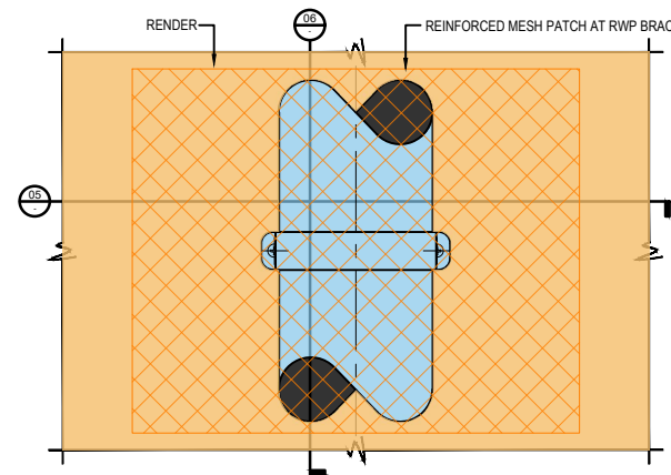
04 PART ELEVATION - RENDER / EXISTING RWP DETAIL Scale 1:3
