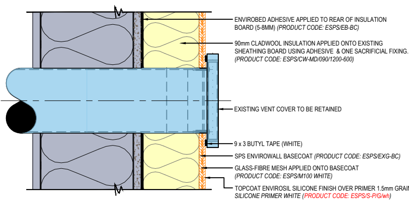
03 CROSS SECTION - RENDER / EXISTING VENT DETAIL Scale 1:3
