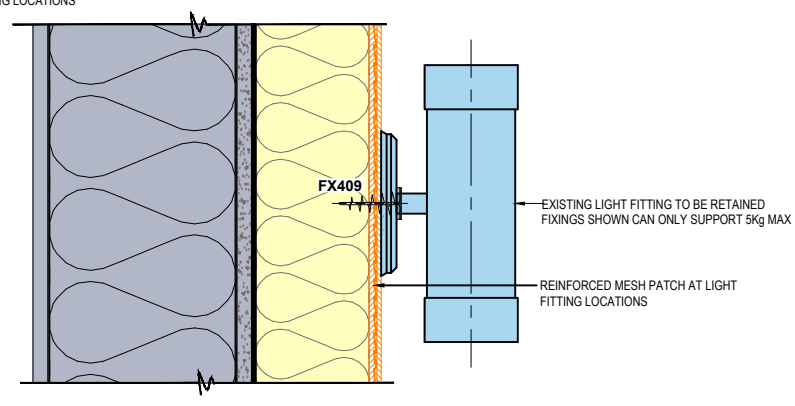
09 CROSS SECTION - RENDER / EXISTING LIGHT DETAIL Scale 1:3
