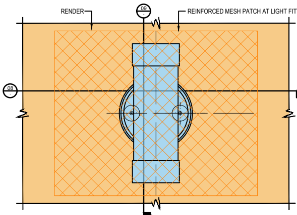
07 PART ELEVATION - RENDER / EXISTING LIGHT DETAIL Scale 1:3
