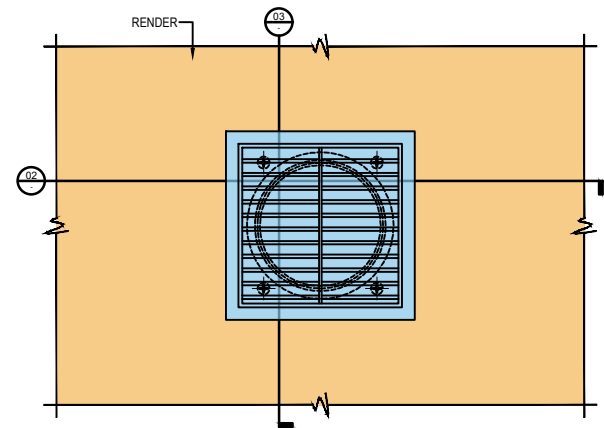
01 PART ELEVATION - RENDER / EXISTING VENT DETAIL Scale 1:3
