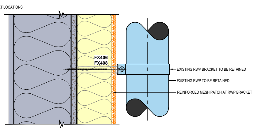
06 CROSS SECTION - RENDER / EXISTING RWP DETAIL Scale 1:3
